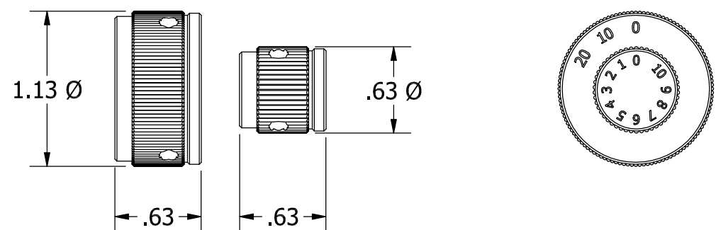
KNOB DETAIL
