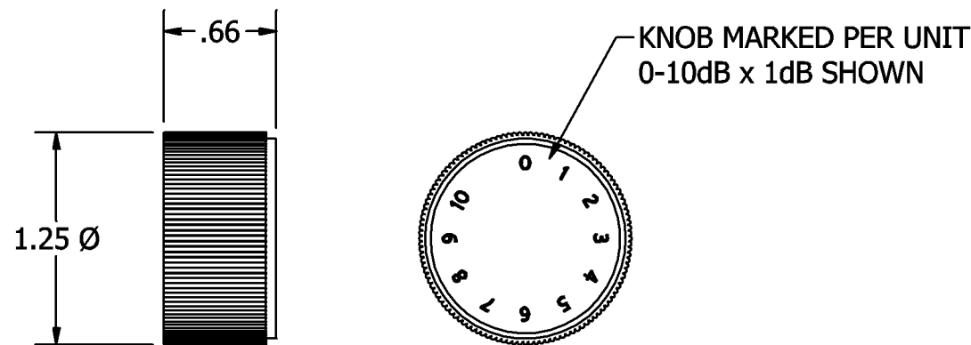
KNOB DETAIL
