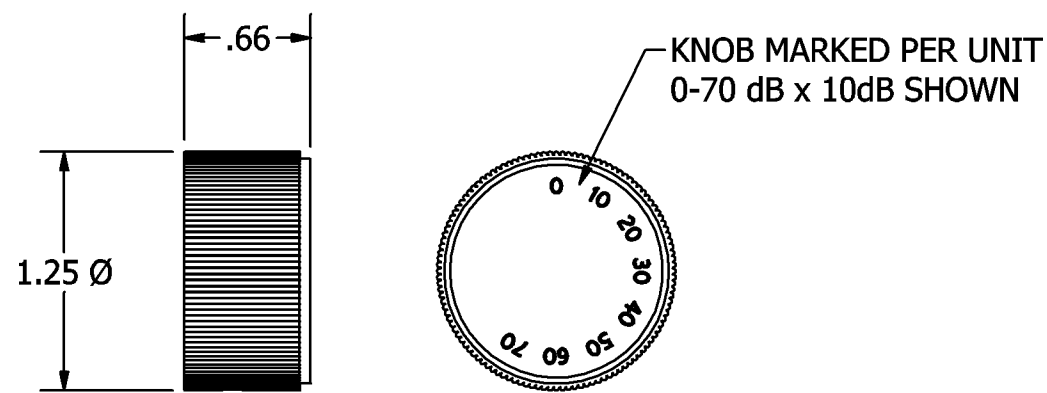
KNOB DETAIL
