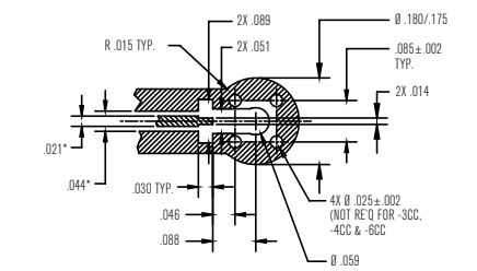
Mounting Hole Pattern
