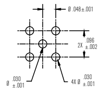
Recommended Mounting Hole Pattern
