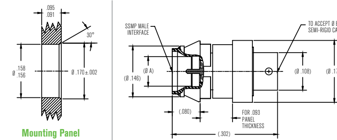
Mounting Panel Scale: None
