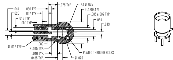
Mounting Hole Pattern
