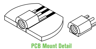
PCB Mount Detail
