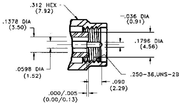
Male Plug
