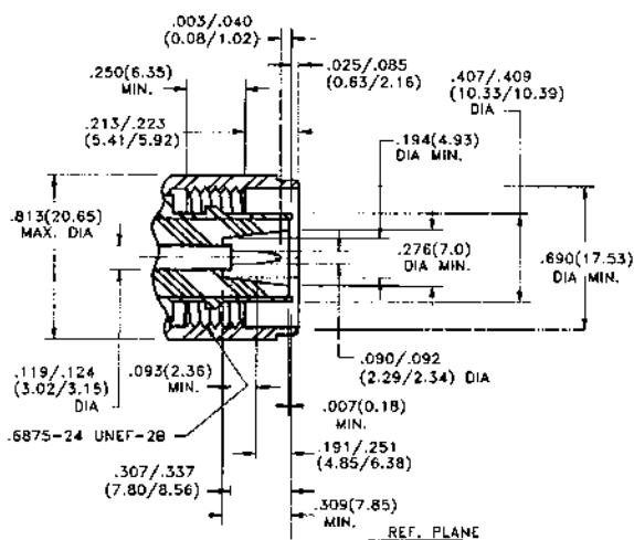
Male Plug
