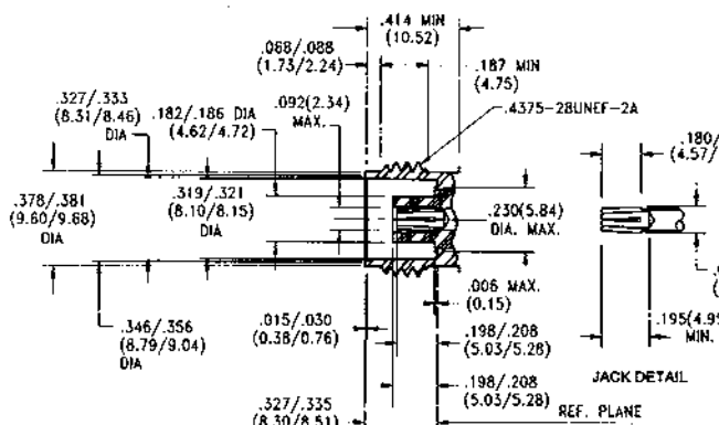
Female Jack
