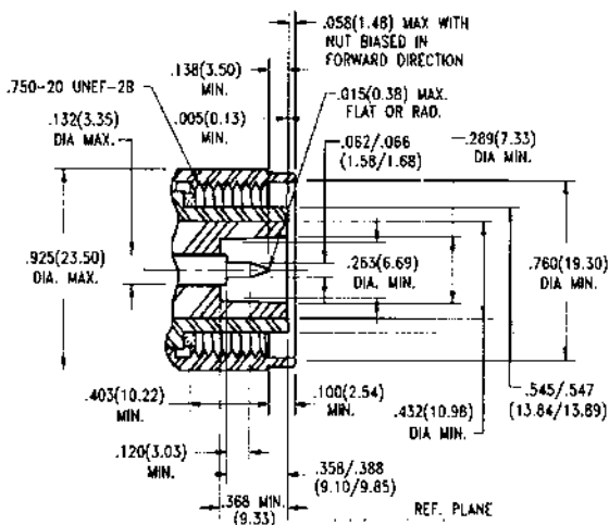
Male Plug
