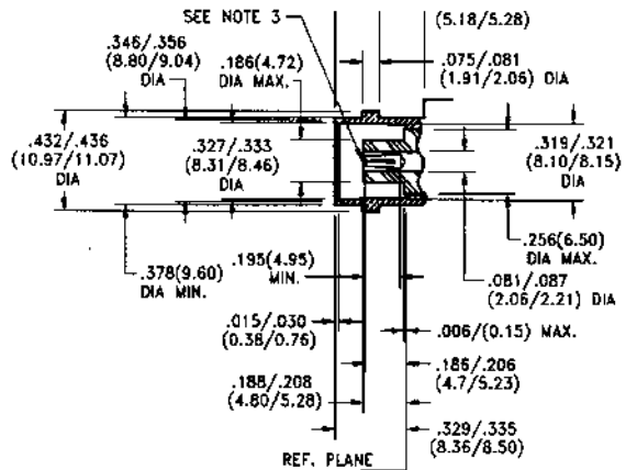
Female Jack
