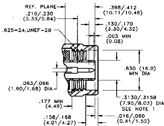
Male Plug
