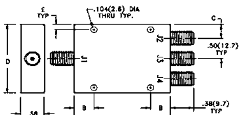
Case Style 1
