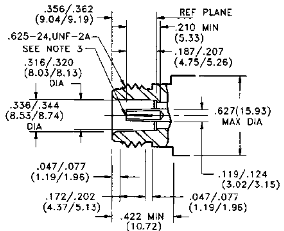
Female Jack
