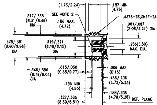
Female Jack
