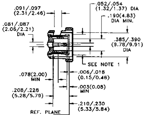
Male Plug
