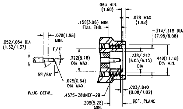
Male Plug
