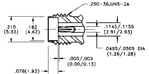
Female Jack
