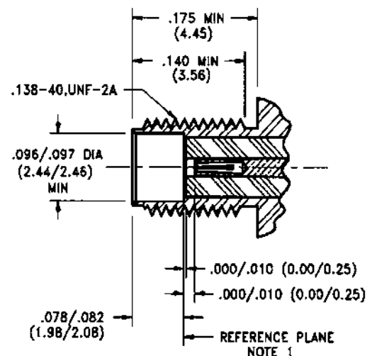
Female Jack
