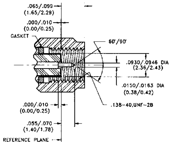
Male Plug
