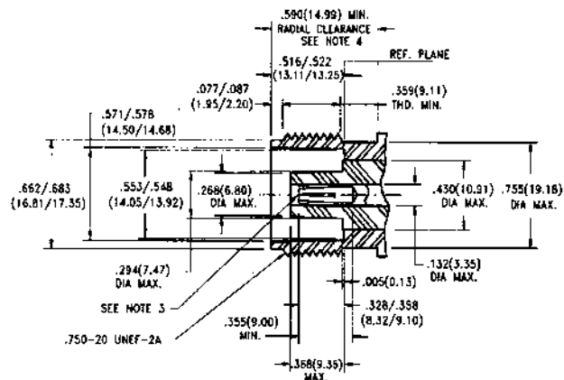
Female Jack
