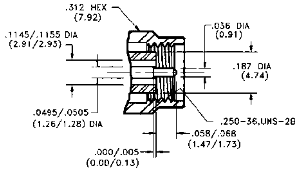
Male Plug
