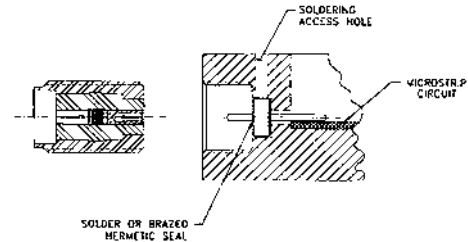
Drop-in Assembly - Feedthru Connector
