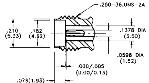
Female Jack
